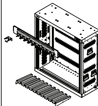
Model: MWRM203/M500 10 M203 or shotguns 42"W x 16.25"D x 45"H
