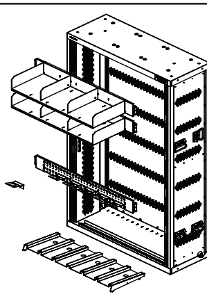
Model: MWRM240SH 6 M280B's 42"W x 16.25"D x 84"H
